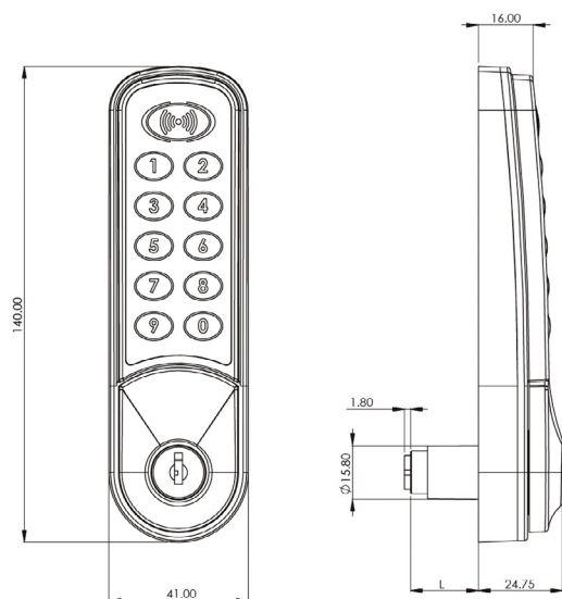
RFID NIMBUS SURFACE MOUNT
